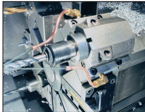
JetTubes shown on CNC turning center.
